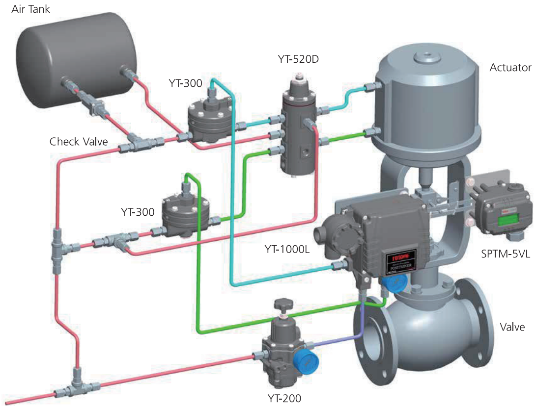
YF1000L (Double type) Application Example
