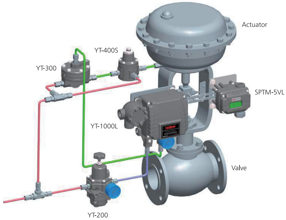
YF1000L (Single type) Application Example
